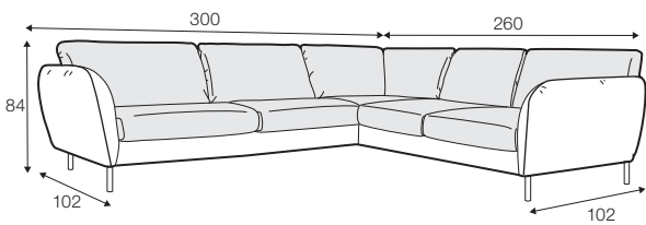
set 8 3 seater left / or right + corner 90° no1 + 2 seater right / or left
